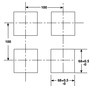
PANEL CUT-OUT
